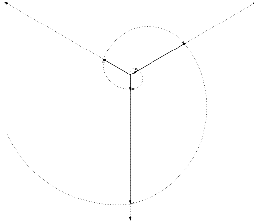
FIGURE 2. The path traced by f(i) = \left(\frac{3}{2}\right)^i intersecting with m = 3 concurrent rays.
