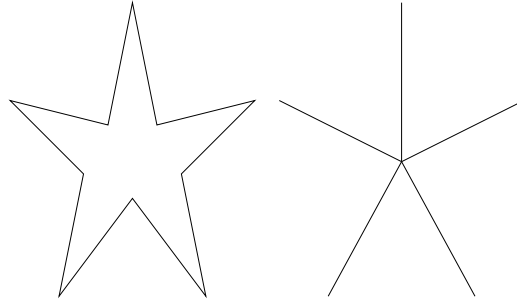
FIGURE 1. The representation of a star shaped polygon by a set of rays all co-terminal. This can be thought of as a potential search path.
