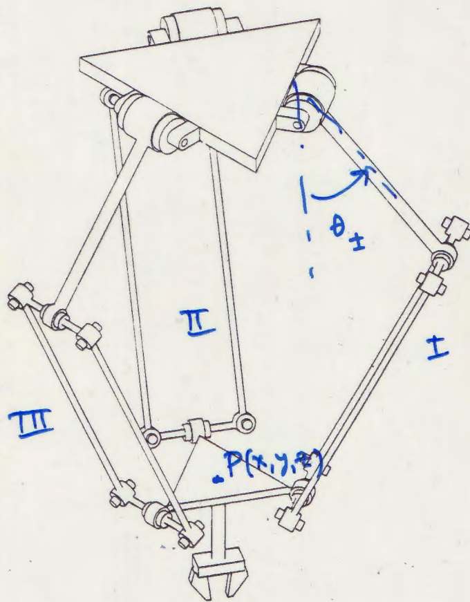
FIGURE 1.6. The Clavel Delta robot.
