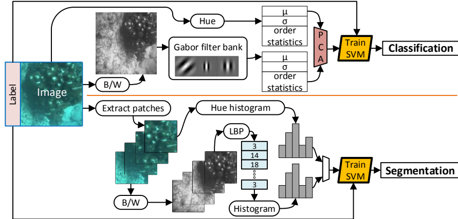
Fig. 3: Image processing pipeline. (top) Gabor-based classification. (bottom) LBP-based segmentation.
