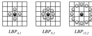
Fig. 4: Local binary pattern neighborhood sets for (P = 4, R = 1) , (P = 8, R = 1) and (P = 12, R = 2) .
