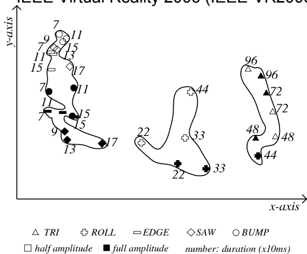
Figure 4: Ordinal untied MDS plot from the average dissimilarity matrix obtained with the cluster-sorting experiment ( stress = 0.083 ). Signal durations (from Table 1) have been rounded to the nearest multiple of 10ms for clarity.
