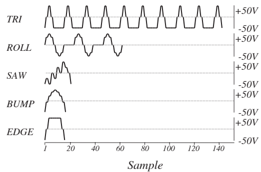
Figure 3: Five waveforms used for the experiment.
