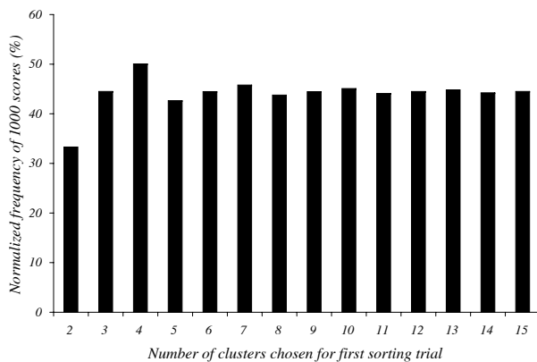
Figure 7: Average normalized frequency of 1000-scores obtained in a randomized cluster sorting execution, as a function of the number of clusters chosen for the first trial. Frequency indicates a proportion of the 435 score-elements present in a 30-stimulus dissimilarity matrix.
