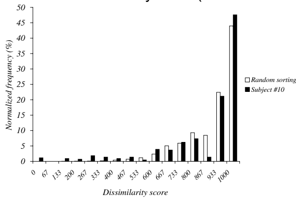
Figure 6: Score distributions for a typical subject and random sorting. Frequency indicates a proportion of the 435 score-elements present in a 30-stimulus dissimilarity matrix.
