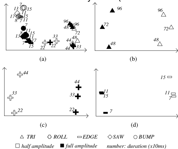
Figure 8: Ordinal untied MDS plots obtained from grouping the different waveforms into cluster-sets of {2,3,4}: (a) control with all 30 stimuli and with isolated (b) TRI, (c) ROLL and (d) EDGE stimuli.
