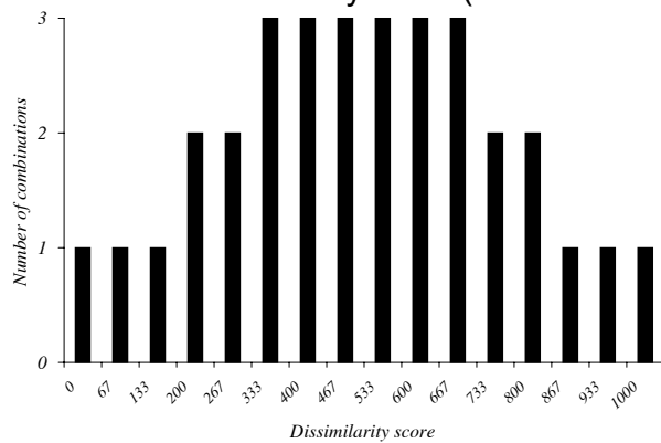
Figure 5: Number of possible combinations to obtain a single dissimilarity score with a cluster-set of {3, 6, 9, 12, 15}.
