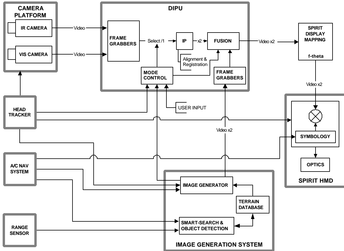
Figure 2. ESVS system architecture
