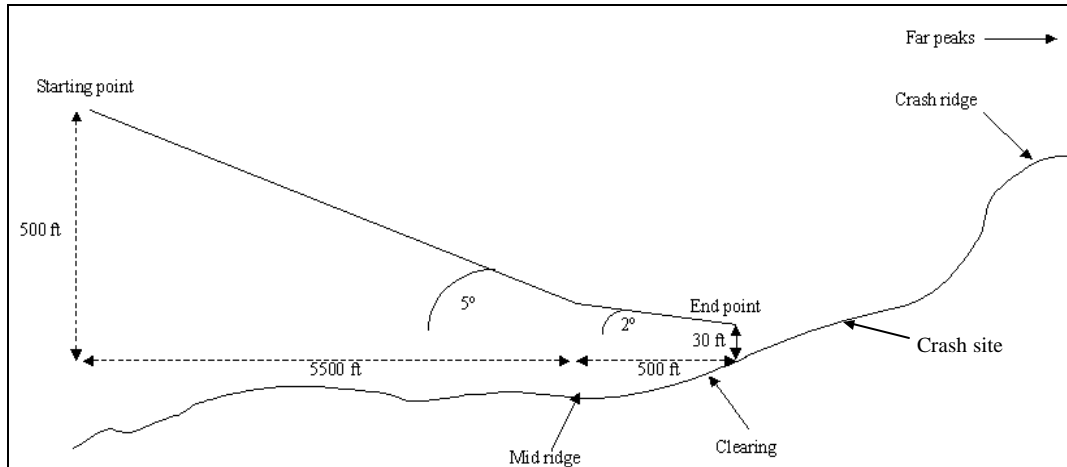
Figure 4. Flight path and terrain profiles
