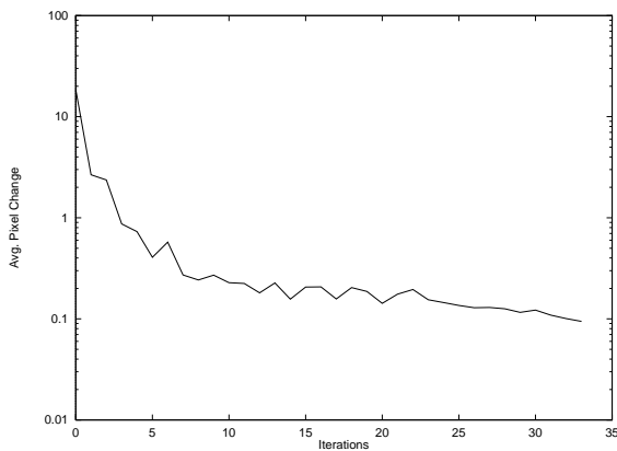
Fig. 9. Graph of the Convergence of The Pyramid Scene
