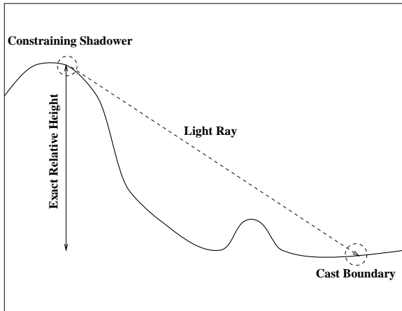
Fig. 5. Exact Relationship Between Heights of Shadow Pairs
