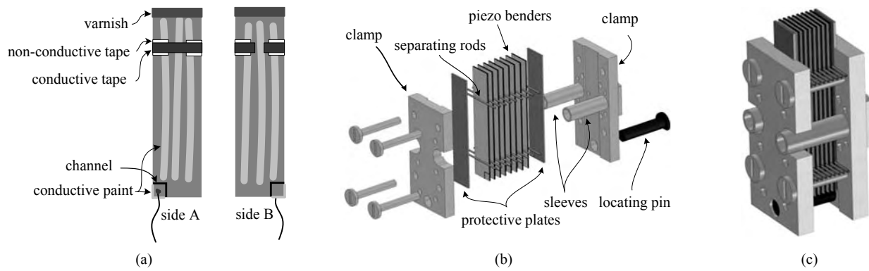
Fig. 6. Building the transducer: (a) preparation of the piezoelectric actuators, (b) assembly and (c) ready to be mounted to the slider.
