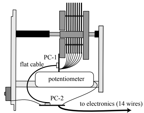
Fig. 9. Wire management.
