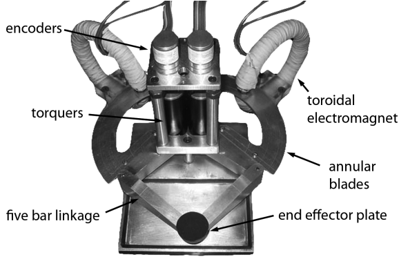
Fig. 2. Hybrid Pantograph with twin eddy current brakes.
