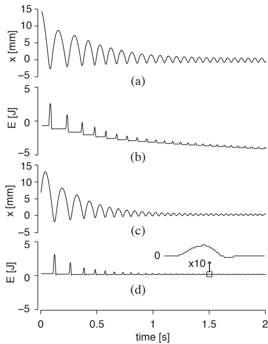
Fig. 8. Results using a virtually damped passivity controller. Undamped 1.5 \text{ N}\cdot\text{mm}^{-1} virtual wall (a) and (b). Wall at 1.5 \text{ N}\cdot\text{mm}^{-1} with virtually damped Passivity Controller (c) and (d). The limit cycle is made more visible by enlargement in the bottom panel.
