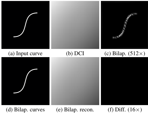
Figure 4: Curves extracted from the image Bilaplacian domain.
