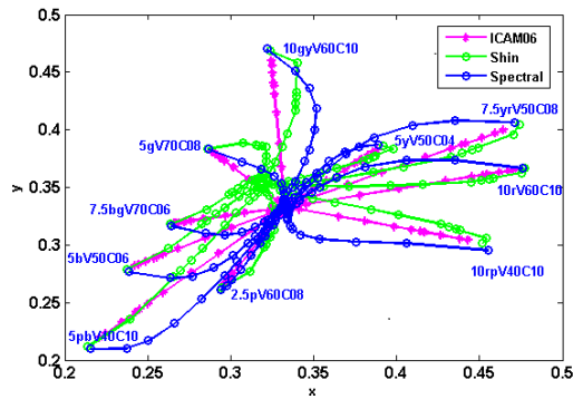
Figure 5: The chromaticity output of iCAM, Shin and Spectral model is shown for 10 different color patches under various luminance values.
