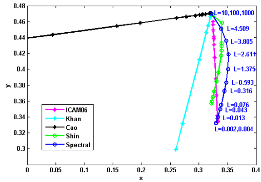
Figure 3: Outputs of different mesopic or scotopic models for a single Munsell patch under different light intensities
